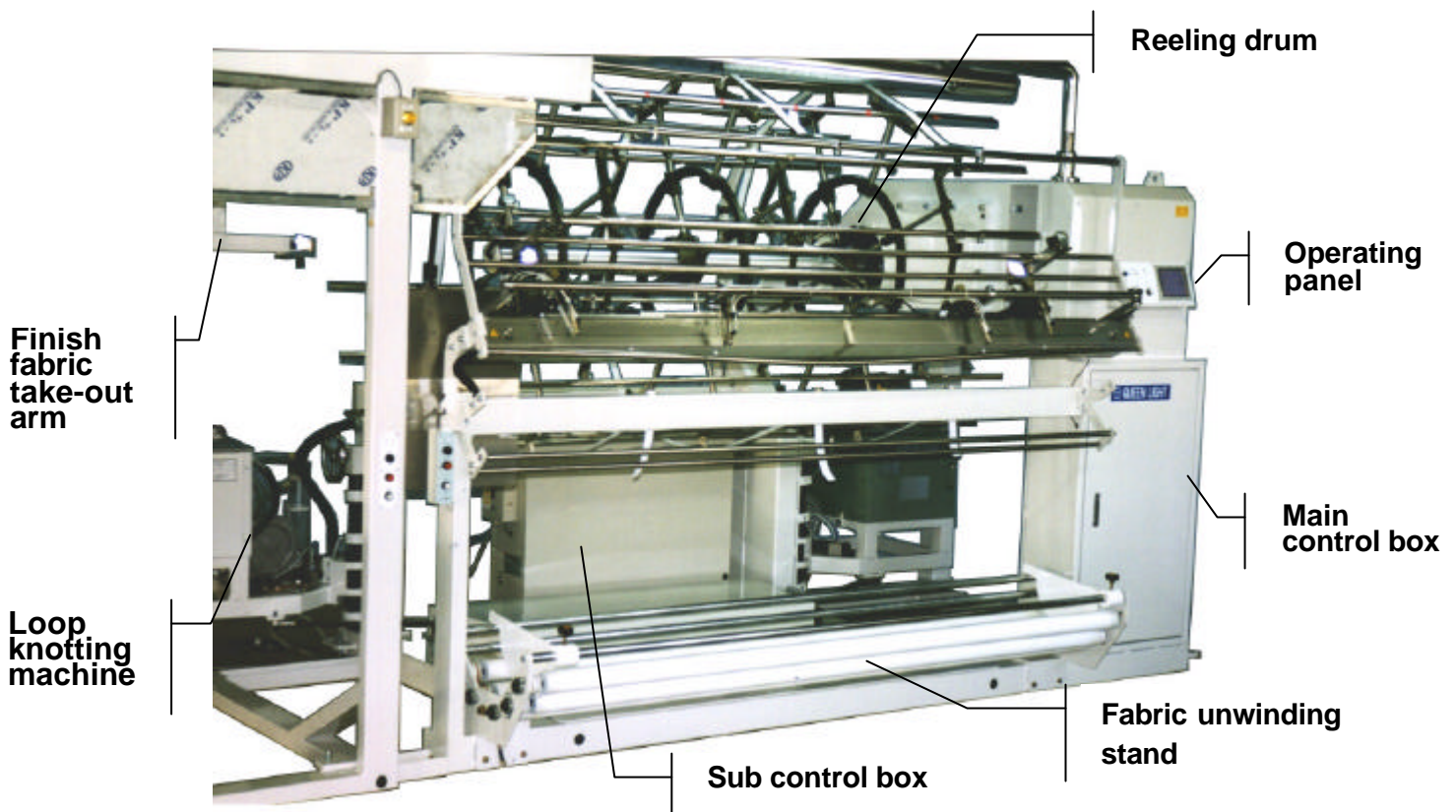
Finished fabric take-out device KSW-2 (Option)
